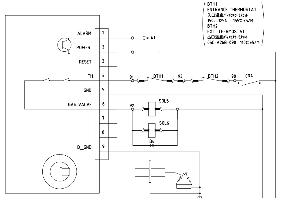
DIRECT SPARK IGNITION CONTROLS FENWAL 35-405200-001
